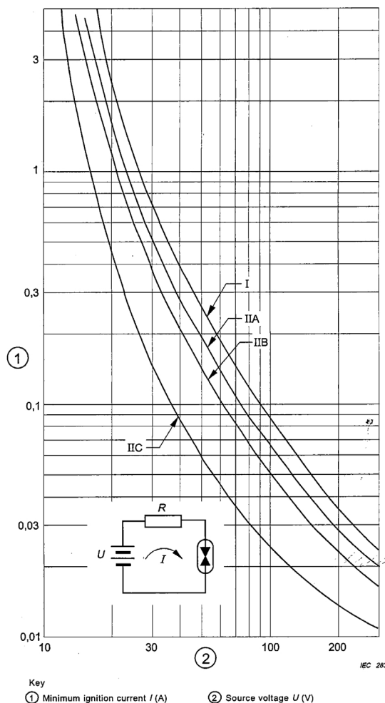
Figure A.1 - Resistive circuits
